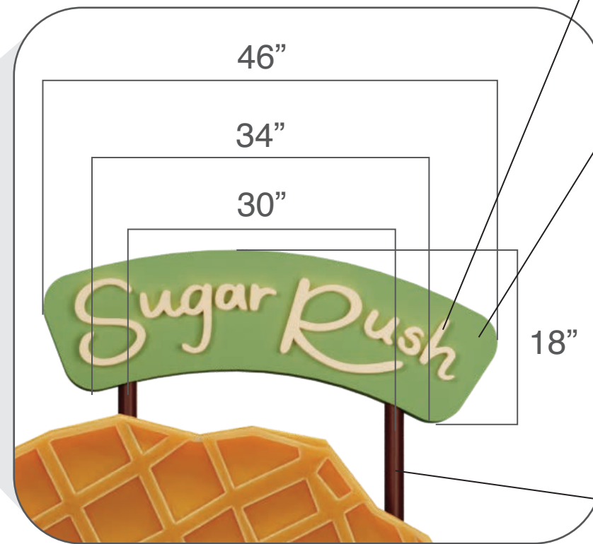
3 A.05 UPPER SIGN DETAIL: FRONT NTS
