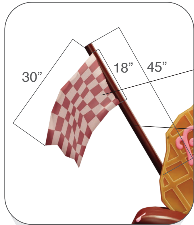
1 A.05 FLAG DETAIL: FRONT NTS
